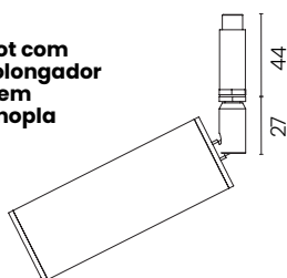
Spot com canopla
